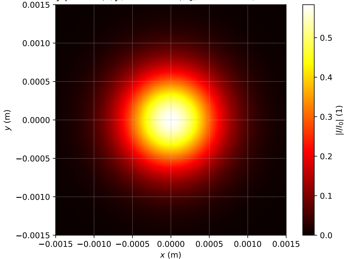
Intensity profile I(x, y, z = 2.548m)/I_0 , \text{Pin}=0.4\text{Pcr} , artificial time
